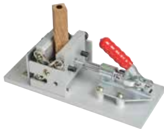
CARBATEC Quick Action Self-Centring Pen Blank Drilling Jig Part No. CT-PV4
