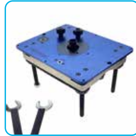
CARBATEC Lift N Lock Router Lift Suits fixed base routers Part No. RT-LIFT-FB
